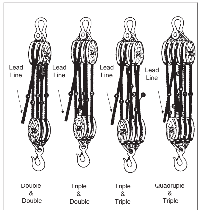
Reeving Diagram
